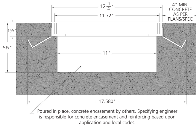
Heavy Duty Stainless Steel Subway Bar Grates
