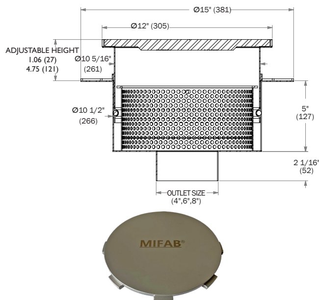
Special duty solid cover with perimeter drain gap (-PD)
