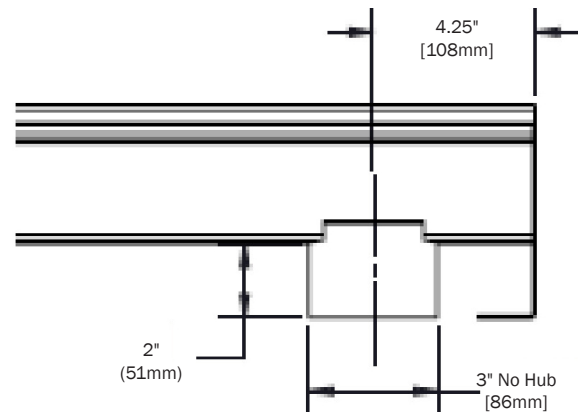
3" No Hub bottom outlet detail
