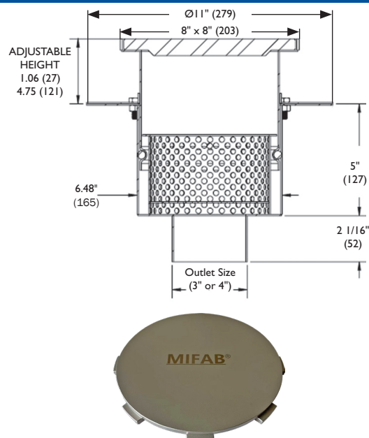
Special duty solid cover with perimeter drain gap (-PD)
