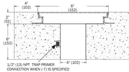
P6460-THTD cross section
