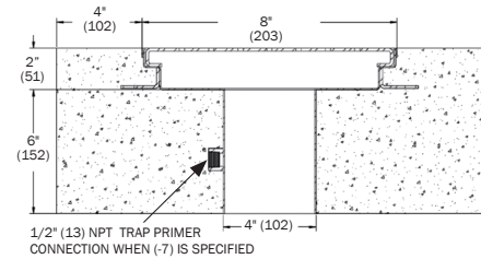
P6480-THTD cross section
