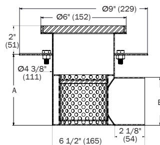
Optional -90 side outlet (with non-adjustable top)
