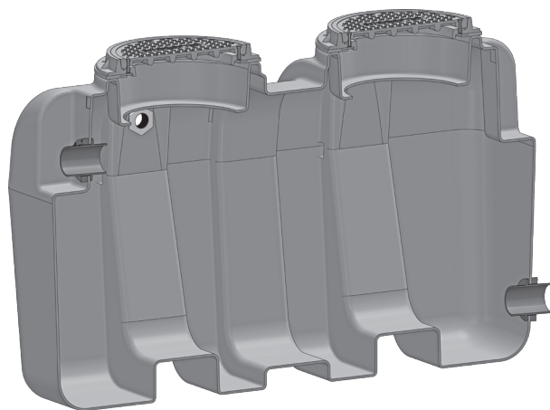
BIG-DECON 55, 140 and 300 Gallons Decontamination Tank
