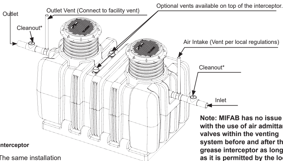
Part number for the 4" vent connection is BIG-PF4
