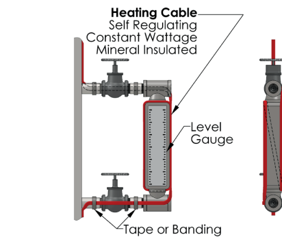
AD12 - Level Gauge
