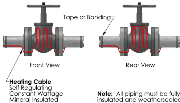
AD9 - Valve
