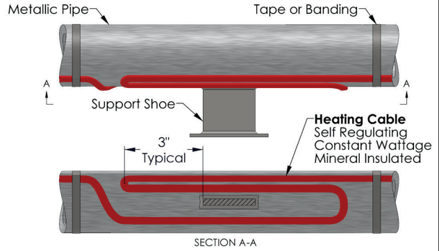
AD8 - Shoe Support
