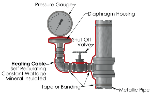
AD11 - Diaphragm Pressure Gauge
