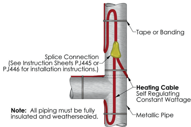
AD14 - EL Series Splice and Tee Kit
