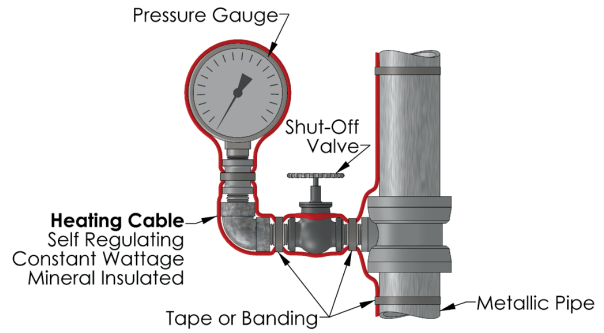
AD10 - Pressure Gauge
