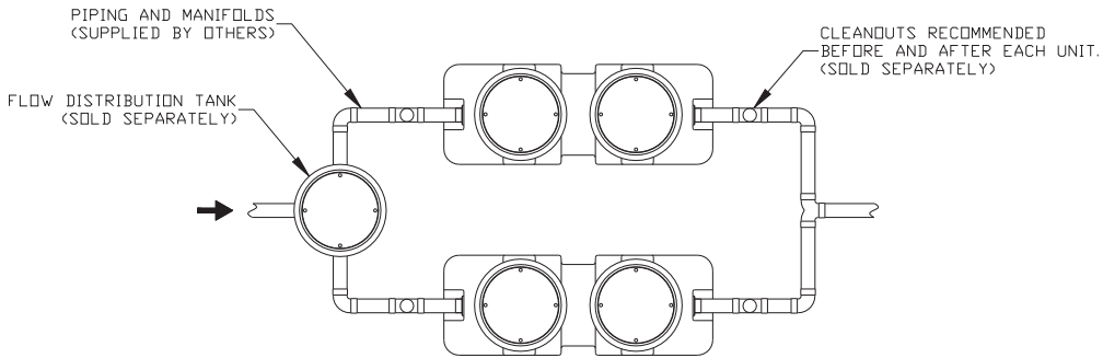
XL-MI-G-PL-1150 TWO IN PARALLEL 200 GPM, 2300 GREASE LBS. CAPACITY
