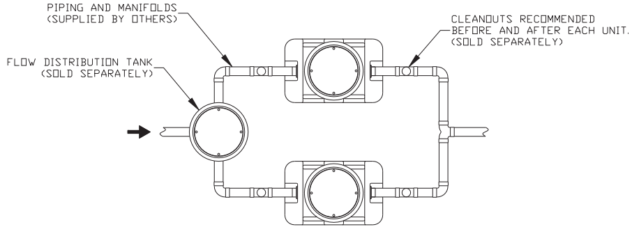
XL-MI-G-PL-750 TWO IN PARALLEL 150 GPM, 1500 GREASE LBS. CAPACITY
