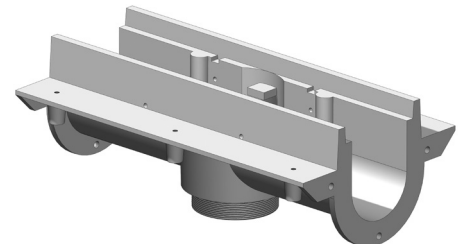
T1320T-FLC-PB - Bottom Outlet Section (Specify any A1 body to make outlet connection)
