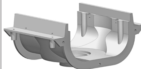
T1350T-FLC-PB - Bottom Outlet Section (Specify any A1 body to make outlet connection)
