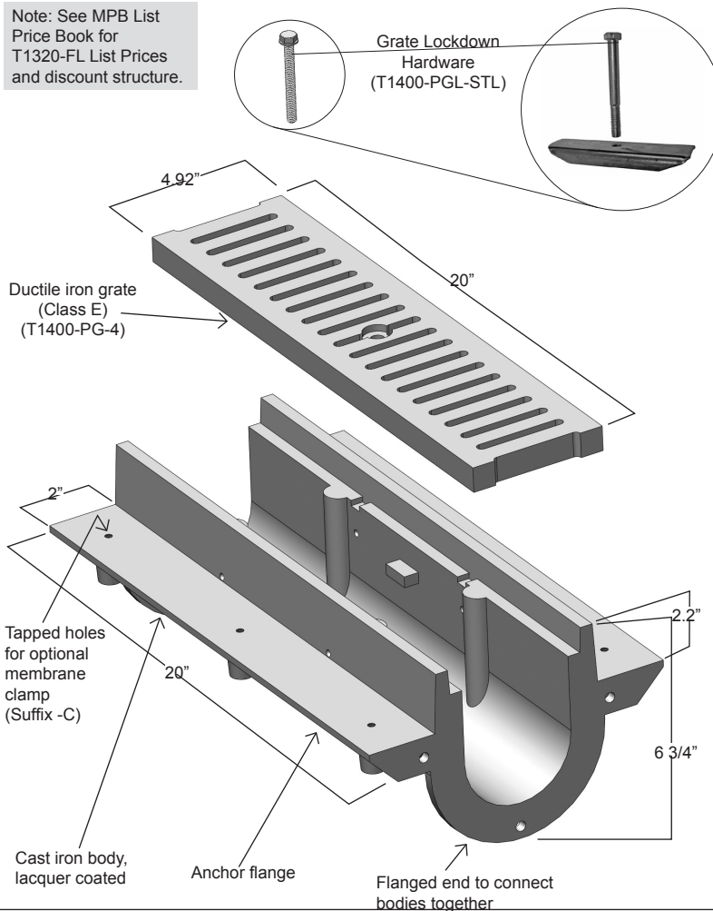
T1320T-FLC-PB - Bottom Outlet Section (Specify any A1 body to make outlet connection)
