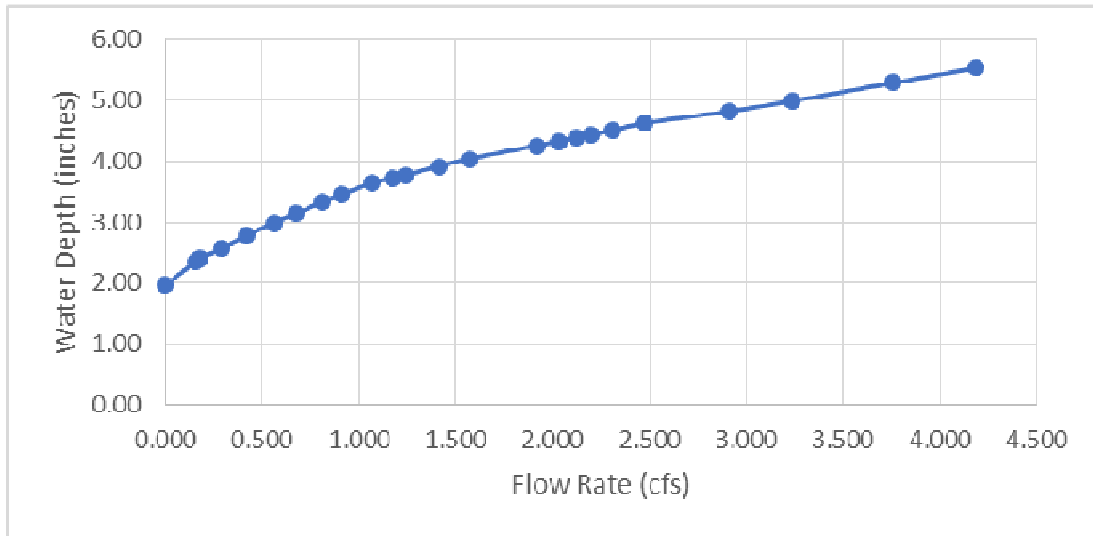
Figure 1, Rating curve
