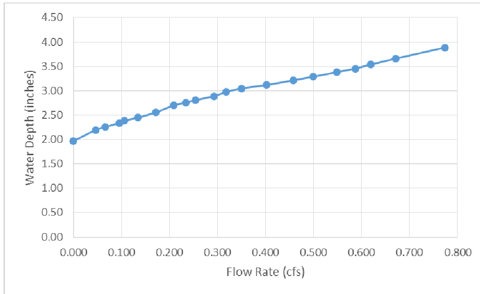
Figure 1, Rating curve
