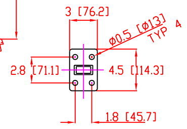
BASE DETAIL
