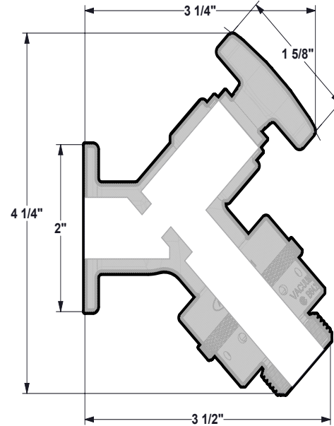
HY-9000 Series wall faucet dimensions
