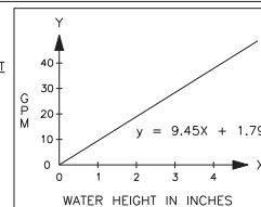
WEIR FLOW DATA CHART
