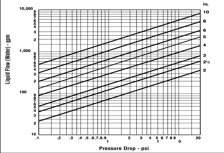
Flow/Pressure Drop Chart
