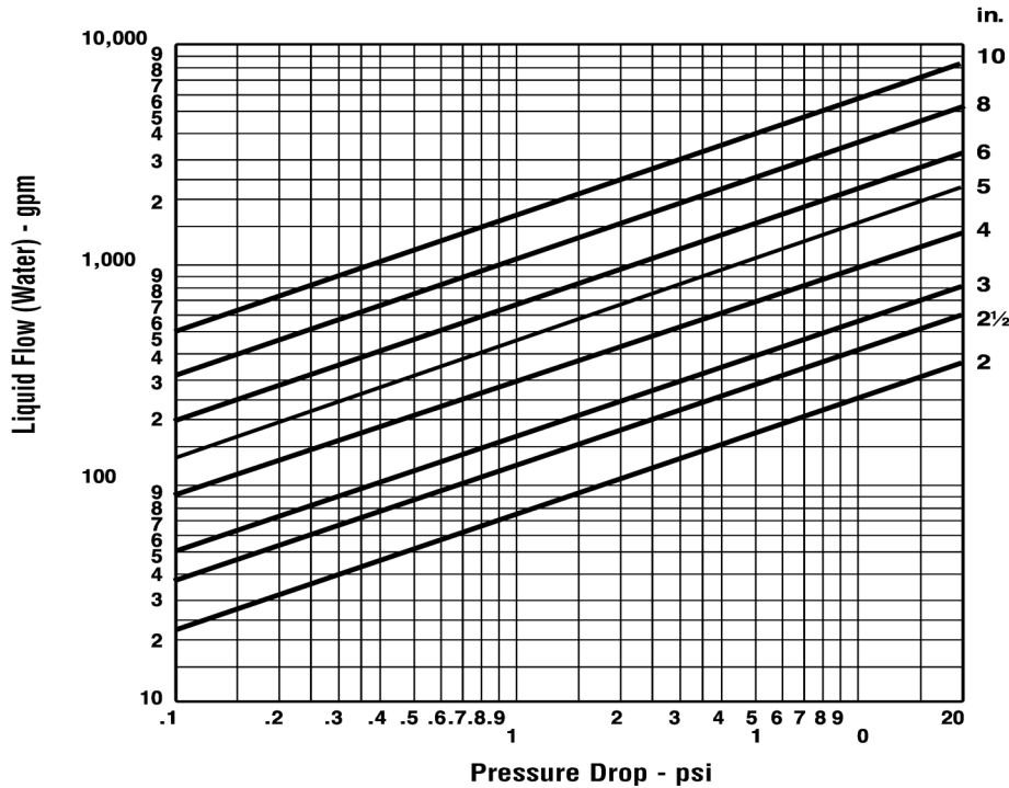
Flow/Pressure Drop Chart
