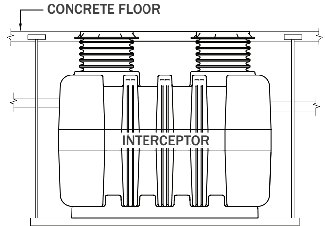
SUSPENDED INSTALLATION
